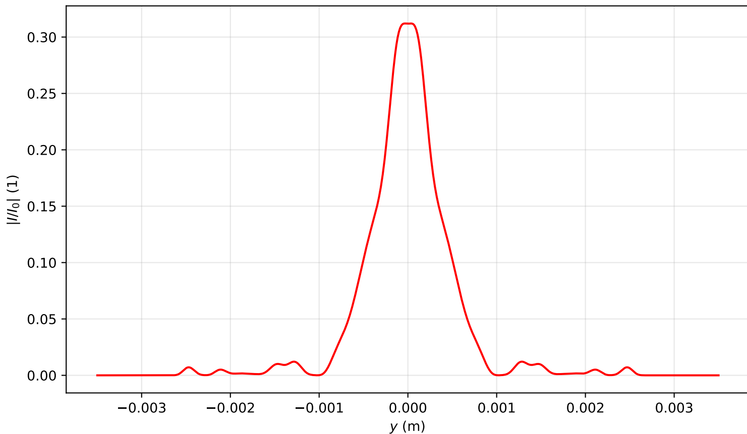
Intensity profile I(x=0, y, z=2.070)/I_0 , P_{in}=4.0P_{cr} , artificial time
